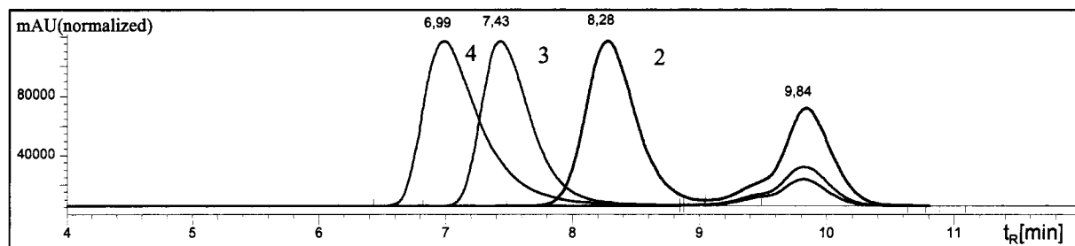
Figure 8. LACCC chromatograms of PtBMA- b -PMMA 2, 3, and 4. (precursor PtBMA, M_n = 73\,000 g/mol) with different PMMA block lengths at critical conditions of PtBMA.
