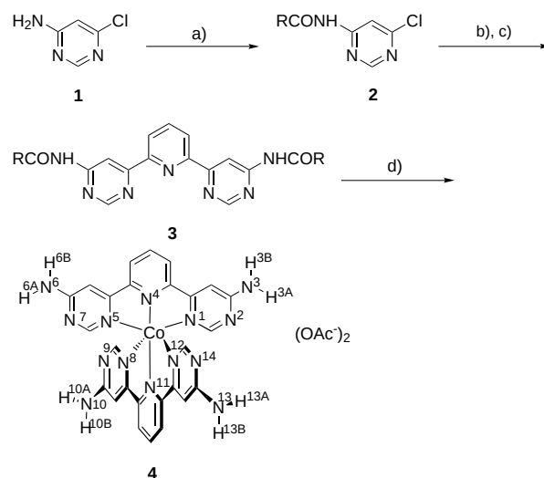
Scheme 2. Synthesis of ligand 3 and Co complex 4 . a) CH_3(CH_2)_4COCl , pyridine, CHCl_3 ; b) Me_6Sn_2 , [Pd(PPh_3)_4] , toluene; c) 2,6-dibromopyridine, [Pd(PPh_3)_4] , toluene; d) Co(OAc)_2 \cdot 2H_2O , MeOH.
