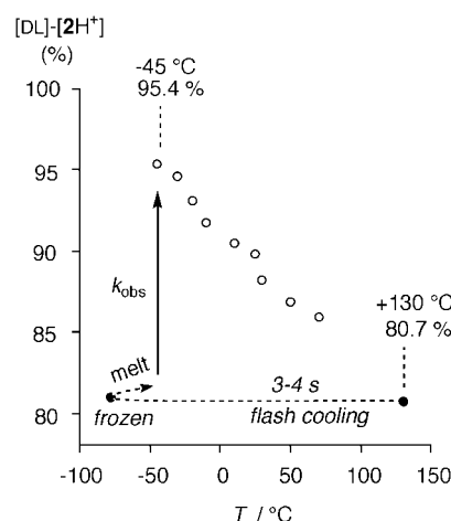
Figure 3. Variation of equilibrium populations of [DL]- ^{13}\text{C} -2H ^+ [I] ^- and [ meso ]- ^{13}\text{C} -2H ^+ [I] ^- in [\text{D}_7]\text{DMF} (as % [DL]-) with temperature (open circles). Filled circles: start ( +130^\circ\text{C} ) and end ( -78^\circ\text{C} ) points for flash cooling ( -\delta T/\delta t \geq 208^\circ\text{C} in 5 s) of dynamic equilibrium population (ca. 80.5:19.5 [DL]/[ meso ]) to static non-equilibrium population (ca. 81.5:18.5) below the freezing-point of the solvent (ca. -62^\circ\text{C} ) used for monitoring kinetics of equilibration by ^{13}\text{C} NMR spectroscopy between -53 and -36^\circ\text{C} , see Figure 4.
