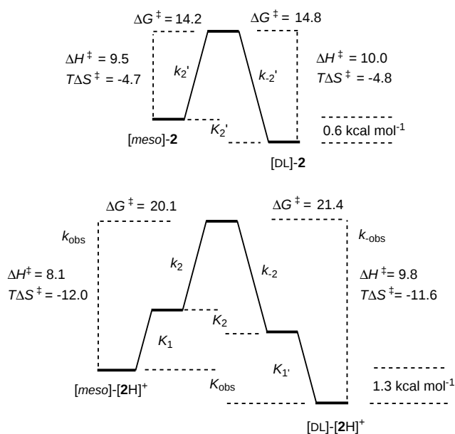
Figure 6. Energy map ( \text{kcal mol}^{-1} ) for stereodynamics of [DL]- and [meso]-[2H + ] (lower section) and [DL]- and [meso]- 2 (upper section). The thermodynamic parameters for 2 (see k_2' and k_{-2}' in Scheme 3) may possibly be used as a crude model for the stereodynamics of non-HB -[2H + ] ( k_2 and k_{-2} in Scheme 3) and thereby gain access to thermodynamic information regarding K_1 in Scheme 3. Note. The vertical dimension ( E ) and horizontal dimension (reaction coordinate) are not to scale and the lines connecting states are merely drawn as an aid for the eye.
