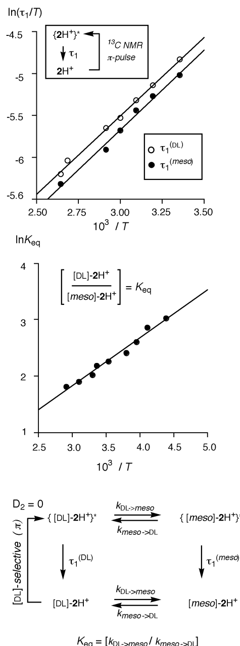
Figure 1. Top: Eyring type analysis of the variation of ^{13}\text{C} NMR (125 MHz) relaxation rate, \tau_1 ( =T_1^{-1} ) of the ^{13}\text{C} -labelled methyl group of [\text{DL}]\text{-}[\text{13C-2H}]^+[\text{I}]^- and [\text{meso}]\text{-}[\text{13C-2H}]^+[\text{I}]^- in [\text{D}_7]\text{DMF} between 25 and 70^\circ\text{C} . Centre: van't Hoff type analysis of the equilibrium populations of [\text{DL}]\text{-}[\text{13C-2H}]^+[\text{I}]^- and [\text{meso}]\text{-}[\text{13C-2H}]^+[\text{I}]^- in [\text{D}_7]\text{DMF} between -45 and +70^\circ\text{C} (by ^{13}\text{C} NMR, 100 MHz).
