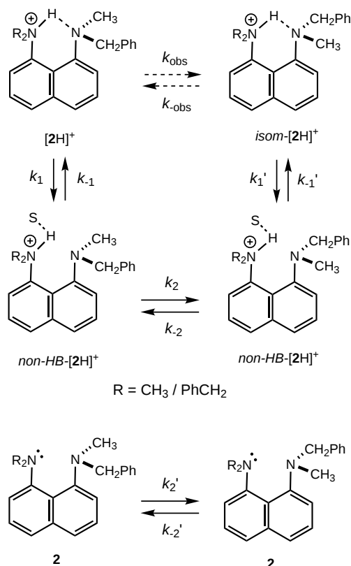
Scheme 3. Model for the interconversion of [DL]-[2H + ] and [meso]-[2H + ] by a two-step process involving solvent-assisted (S = [D 7 ]DMF) hydrogen bond fission ( k_1 ) to give non-HB -[2H + ], followed by rotation-inversion ( k_2 ) and then hydrogen bond formation. The stereodynamics of 2 may possibly be used as a crude model for the stereodynamics of non-HB -[2H + ] ( K_1 in Scheme 3) and thereby gain access to thermodynamic information regarding K_1 in Scheme 3.
