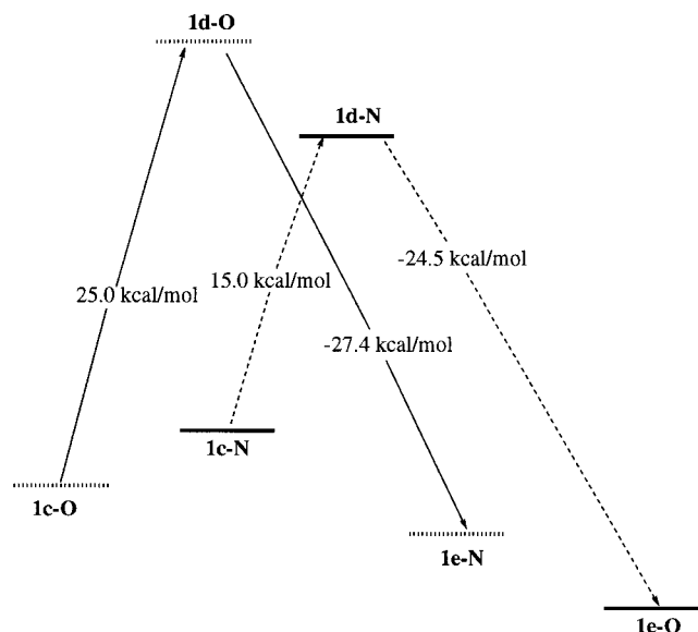
Figure 5. Reaction profile for the insertion of system 1.
