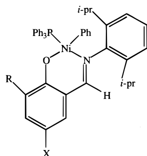
Figure 1. Skeleton structure of the salicylaldiminato nickel(II) complex.
