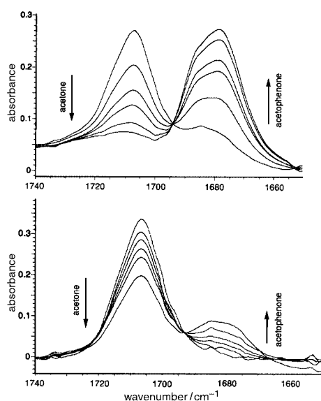
Fig. 2 Dehydrogenation of ( R )- (top) and ( S )-1-phenylethanol (bottom) using ligand 1.
