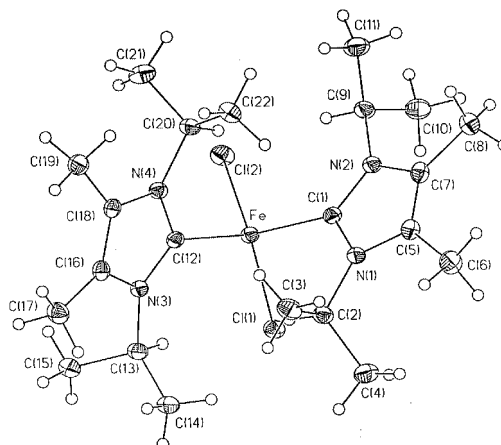
Fig. 1 Molecular structure of complex 1 . Selected bond lengths (Å) and angles (°): Fe–C(1) 2.1363(15), Fe–C(12) 2.1298(16), Fe–Cl(1) 2.3035(4), Fe–Cl(2) 2.2976(4); C(12)–Fe–C(1) 102.05(6), C(12)–Fe–Cl(2) 106.85(4), C(1)–Fe–Cl(2) 114.41(4), C(12)–Fe–Cl(1) 115.62(4), C(1)–Fe–Cl(1) 104.68(4), Cl(2)–Fe–Cl(1) 112.947(17).
