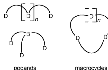
Fig. 1 Topologies of polydentate ligands (D = donor function, B = bridgehead function).
