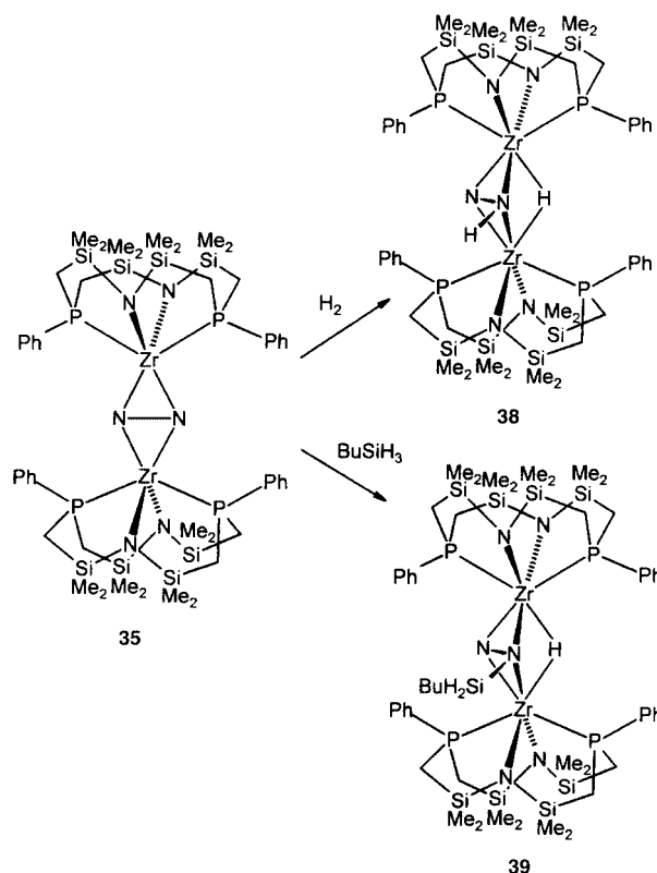
Scheme 5 Hydrogenation of the (μ-N 2 )Zr 2 complex 35 giving the (HN 2 )Zr complex 38 and addition of Bu n SiH 3 to 35 to give the {(BuH 2 Si)N 2 }Zr complex 39 .
