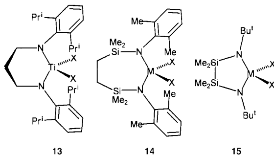
Fig. 8 Group 4 metal complexes containing chelating diamido ligands which are active catalysts for olefin polymerization.
