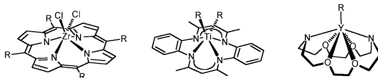
Fig. 2 N-donor macrocycles of different flexibility which have been employed in early transition metal chemistry.
