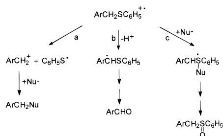
Scheme 18
