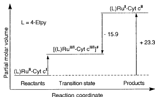
Scheme 7. Volume Profiles for Reaction 18, L = 4-Ethylpyridine
