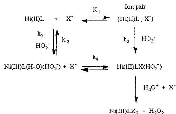
Scheme 1. Mechanism of Oxidation of \text{Ni}^{\text{II}}\text{L} by \text{HO}_2^{\bullet}
