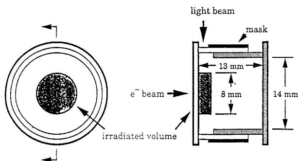
FIGURE 2. Schematic diagram of the pillbox sample cell showing the electron beam and light beam paths and the irradiated volume.
