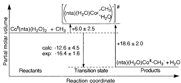
Scheme 3. Volume Profile for the Reverse Reaction 10, \text{M}^{\text{II}}\text{L}(\text{H}_2\text{O})_2 = \text{Co}^{\text{II}}(\text{nta})(\text{H}_2\text{O})_2^- (Volumes in Units of \text{cm}^3 \text{mol}^{-1} )
