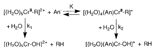
Scheme 5. General Base Catalysis of the Heterolysis of \text{Cr}^{\text{III}}-\text{C} Bonds in [(H_2O)_5\text{Cr}^{\text{III}}-\text{R}]^{2+}
