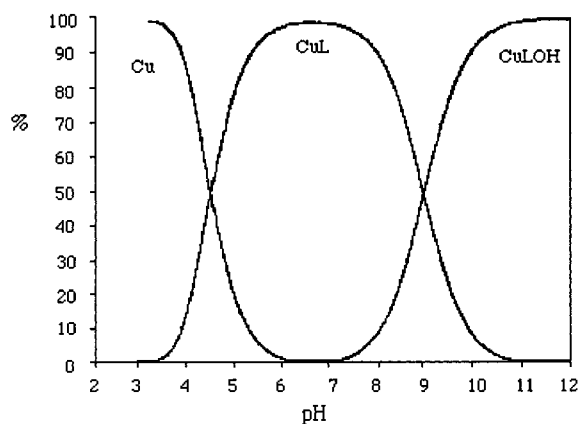
Figure 3. Distribution diagrams of the species formed as a function of pH in the system \text{Cu}^{2+}/\text{L}^2 in a 0.15 M \text{NaClO}_4 solution at 25 °C; [\text{Cu}^{II}] = [\text{L}] = 1 \times 10^{-3} M.
