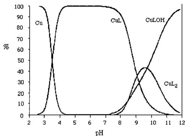
Figure 2. Distribution diagrams of the species formed as a function of pH in the system \text{Cu}^{2+}/\text{L}^1 in a 0.15 M \text{NaClO}_4 solution at 25 °C; [\text{Cu}^{II}] = 1 \times 10^{-3} M, [\text{L}] = 2 \times 10^{-3} M.
