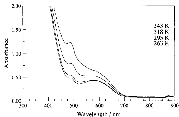
Figure 4. UV-vis spectra at varying temperatures from oxidation of 9 in toluene solution.
