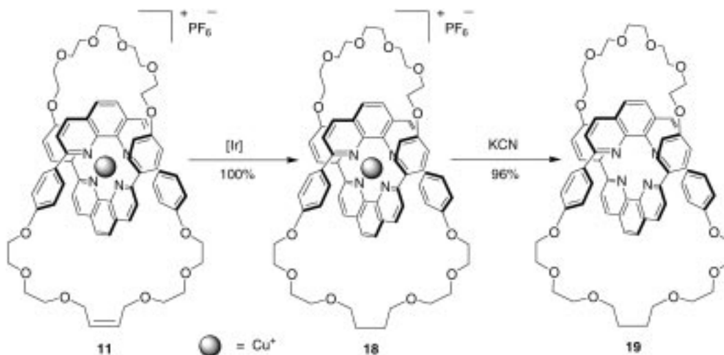
Scheme 6. Hydrogenation of [2]Catenate 9 Using Crabtree's Iridium-based Catalyst To Yield the Double-Bond-Free [2]Catenate 18 Followed by Demetalation To Yield [2]Catenand 19
