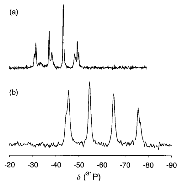
Fig. 2 Solid state CP MAS ^{31}P NMR spectra of (a) [CuCl(PMe_3)_3] , (b) [CuI(PMe_3)_3] .
